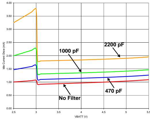
Figure 38. Idle Current Draw vs. VBATT - HD Mode R_L = 8 \Omega + 33 \mu\text{H} (Note 17)
