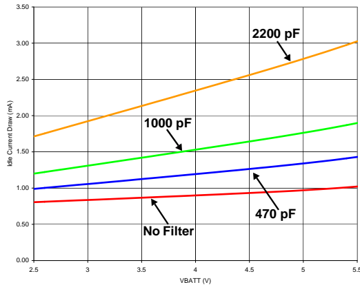
Figure 26. Idle Current Draw vs. VBATT - FSD Mode R_L = 8 \Omega + 33 \mu\text{H} (Note 16)
