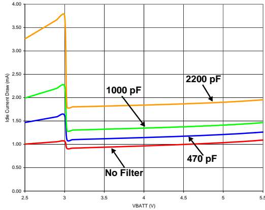
Figure 50. Idle Current Draw vs. VBATT - FHD Mode R_L = 8 \Omega + 33 \mu\text{H} (Note 18)
