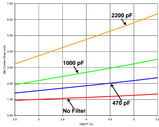
Figure 14. Idle Current Draw vs. VBATT - SD Mode R_L = 8 \Omega + 33 \mu\text{H} (Note 15)
