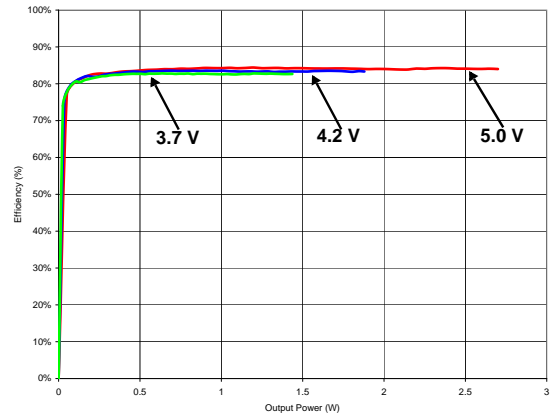
Figure 29. Efficiency vs. Output Power - FSD Mode R_L = 4 \Omega + 33 \mu\text{H}
