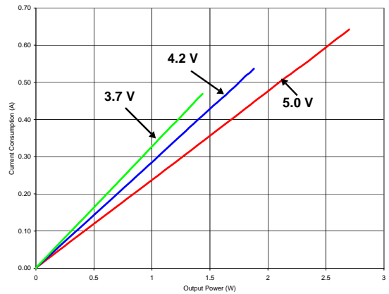
Figure 31. Supply Current vs. Output Power - FSD Mode R_L = 4 \Omega + 33 \mu\text{H}
