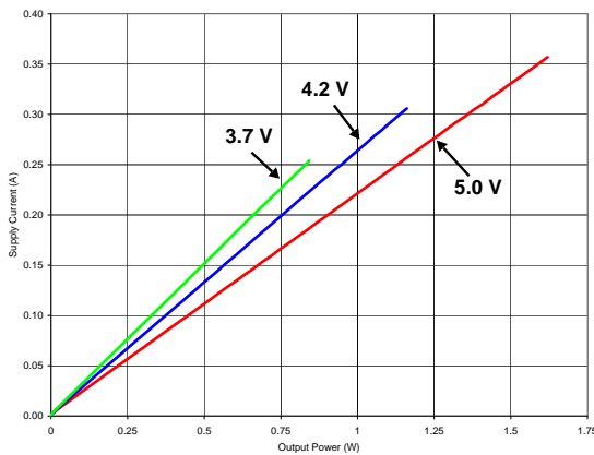
Figure 42. Supply Current vs. Output Power - HD Mode R_L = 8 \Omega + 33 \mu\text{H}
